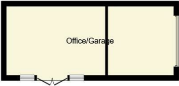
Converted Garage Floor area 20.2 m 2 (217 sq.ft.)
