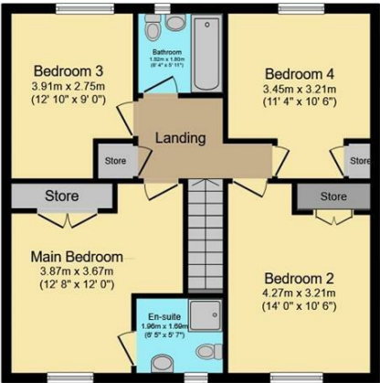
First Floor Floor area 65.3 m 2 (703 sq.ft.)
