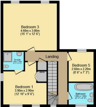
First Floor Floor area 56.0 m 2 (602 sq.ft.)
