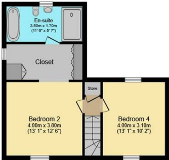
Second Floor Floor area 43.4 m 2 (468 sq.ft.)
