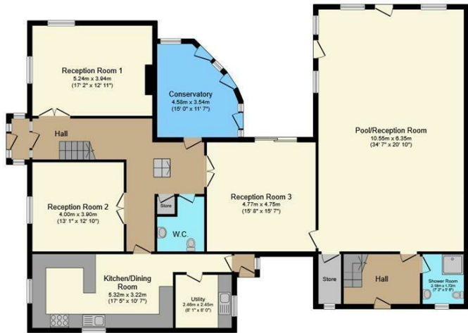
Ground Floor Floor area 212.7 m 2 (2,289 sq.ft.)
