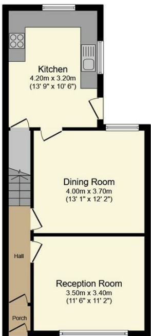
Ground Floor Floor area 49.1 sq.m. (528 sq.ft.)
