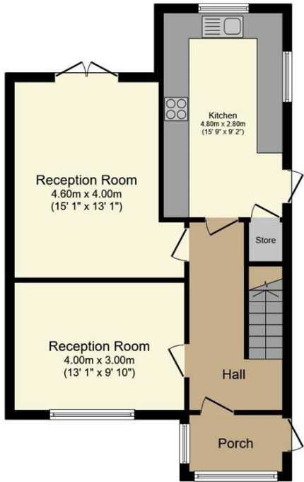
Ground Floor Floor area 56.2 sq.m. (605 sq.ft.)
